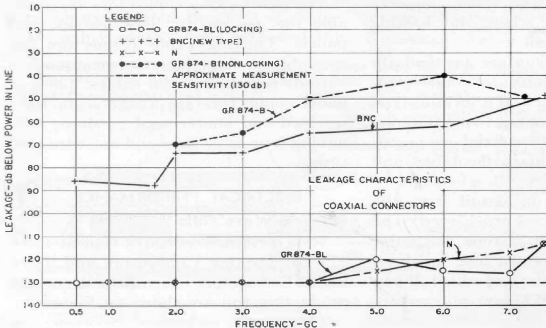
Figure 5. Leakage characteristics of several types of coaxial connectors.
