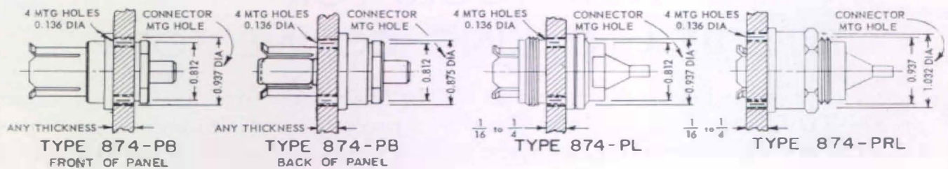
Figure 9. Mounting dimensions for Type 874 Panel Connectors.
