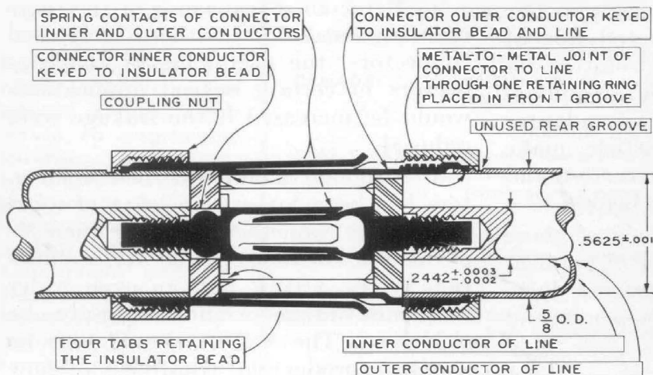
Figure 2. Sectional view of improved non-locking connector. The back edge of the connector outer conductor is drawn up against the retaining ring when the coupling nut is fully tightened. The beveled inside surface of the coupling nut forces the split retaining ring solidly against the bottom of the groove in the outer conductor of the line, and thus a solid metal-to-metal joint is obtained between the outer conductors of the connector and line. The insulating bead is held securely in place by four small tabs which sink into the insulator as the coupling nut is tightened.
