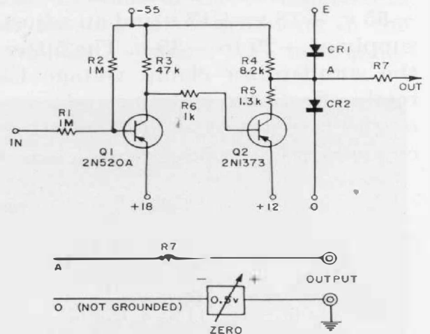
Figure 8. Offset voltage is connected in series with the output terminals.
