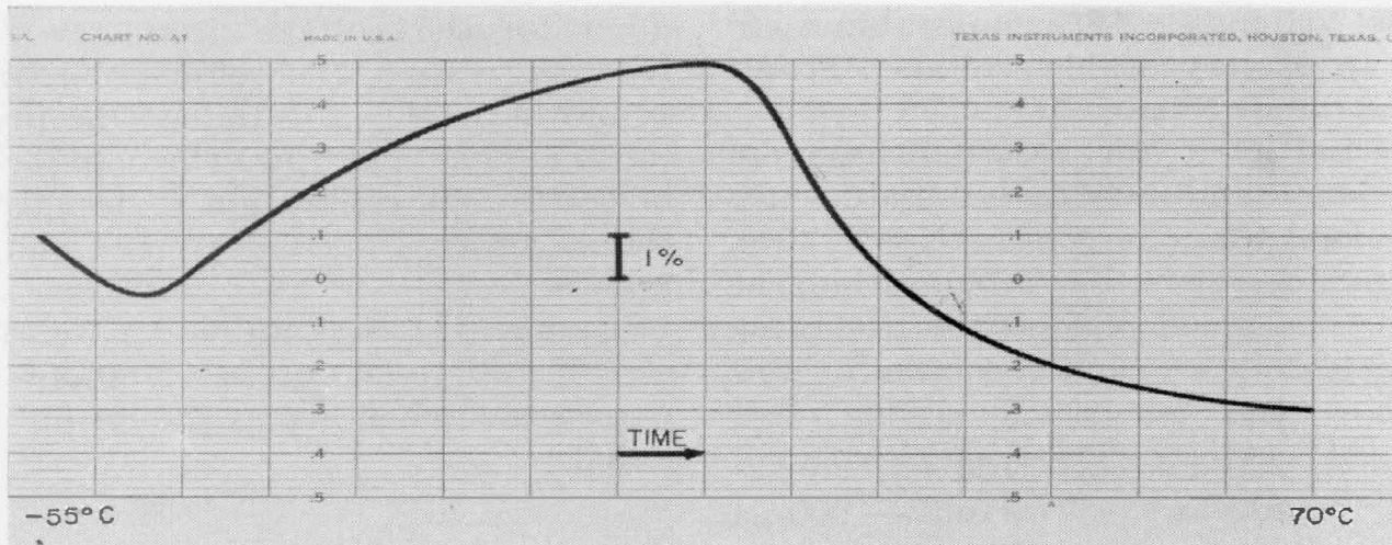
Figure 9. Capacitance-vs-temperature of a capacitor with high dielectric constant. The data were obtained by measuring the period of an RC oscillator.
