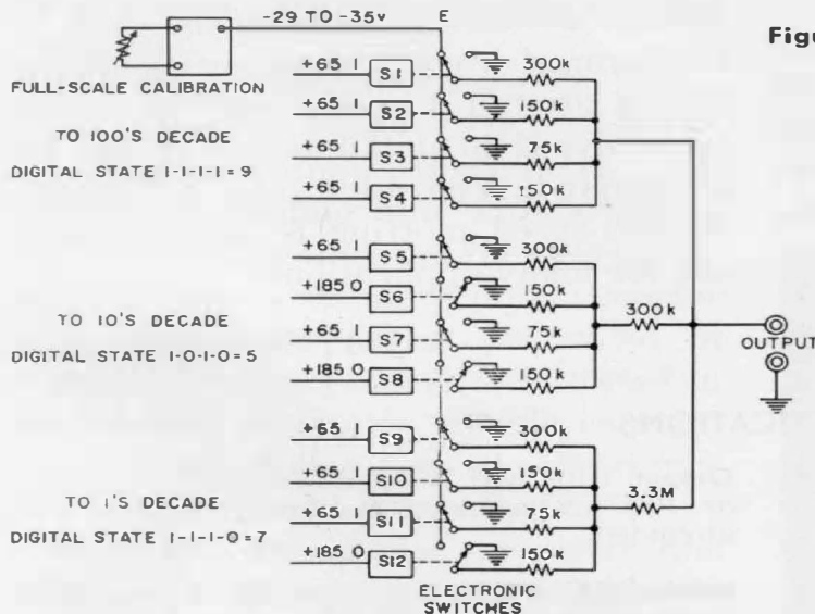
Figure 6. Simplified schematic diagram of the Converter.
