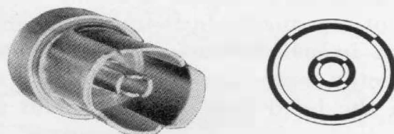
Figure 1. (Left) Type 874 Coaxial Connector. (Right) Cross section of two connectors plugged together.
