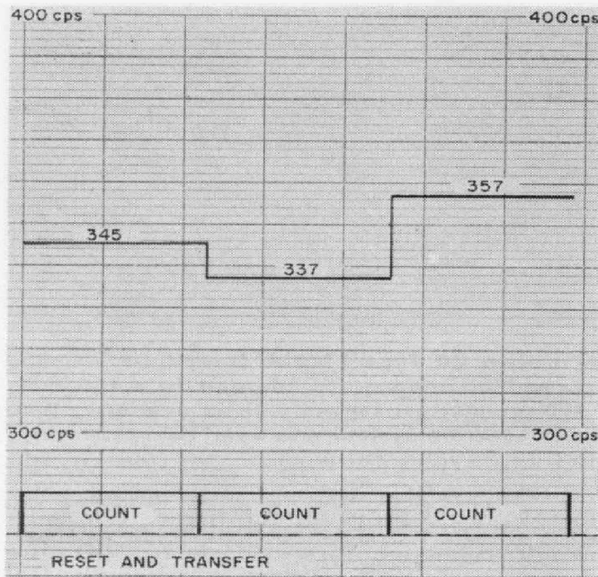
Figure 5. Analog output from 3 storage decades. The output is the result of the previous count.
