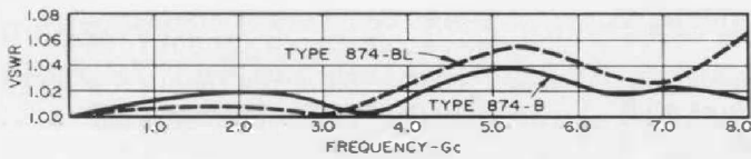
Figure 4. Typical VSWR of Type 874-B and -BL Connectors. Each curve shows the VSWR that a pair of connectors introduces into a line.
