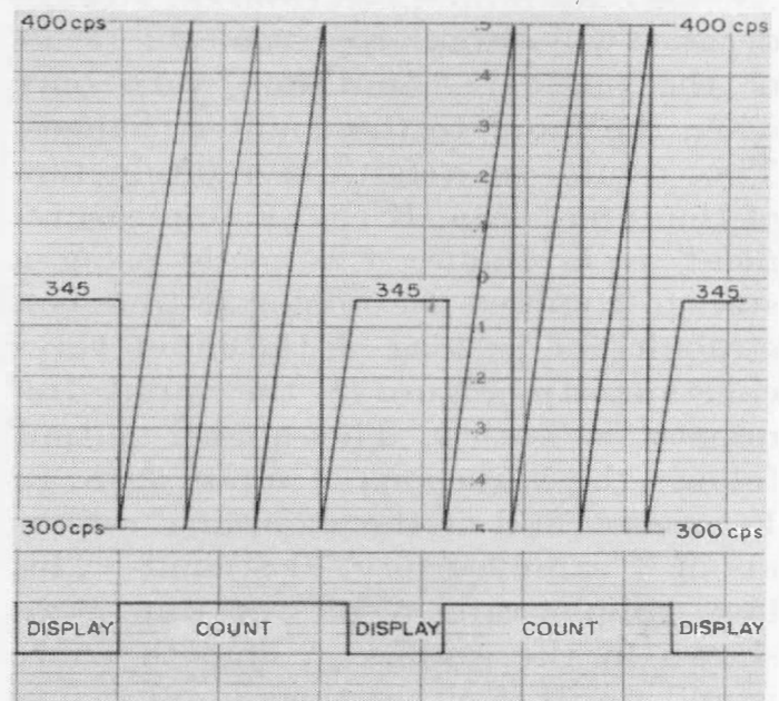
Figure 4. Analog output from 3 conventional decades. Usable information is available during display time only. Gate time was 10 seconds.
