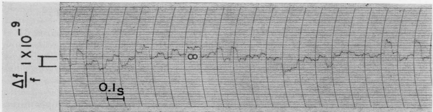
Figure 3. High-speed record of the short-term stability of two GR Type 1113-A Standard-Frequency Oscillators. The 5-Mc outputs are multiplied to 1 Gc each, and the frequency is adjusted for a 105-cycle beat, whose period is recorded. Sampling rate is about 100 samples per second with an averaging time of about 0.01 second. Over-all bandwidth of the measuring system was over 120 cps.
