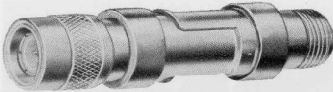
Figure 6. Type 874-QCP and -QNJA Adaptors plugged together. This assembly will connect a Type C jack to a Type N plug.
