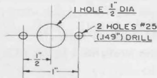
Figure 2. Mounting Dimensions.
